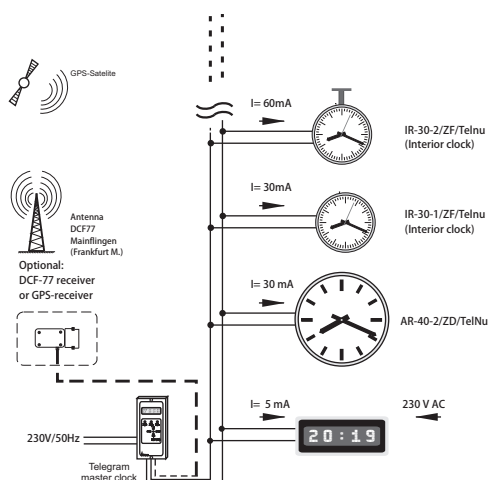
Block diagram for Telegram slave clock system TELNU
